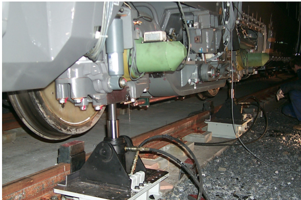
A car buggy shaken by two load units
