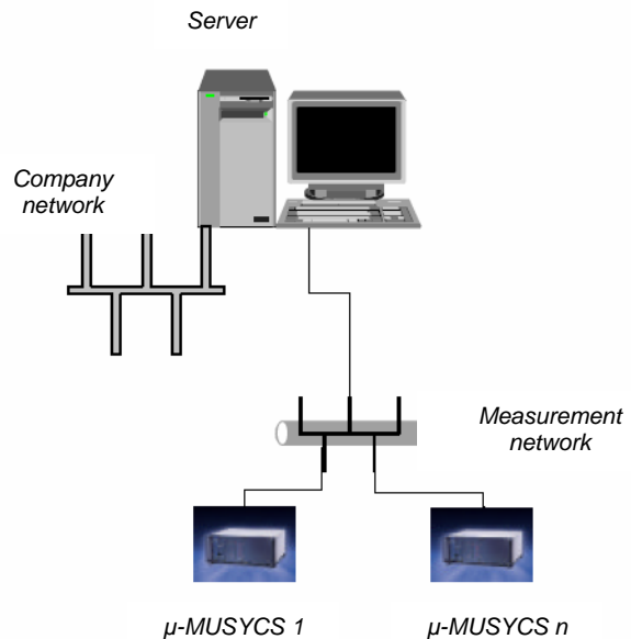
The modular system structure of multiple test rigs
